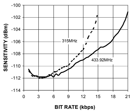
Sensitivity at 1% BER D[4:3] = 01
