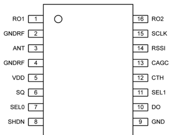
MICRF219AAYQS
