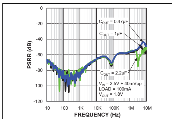
FIGURE 2-11: PSRR (Varying C_{OUT} ).
