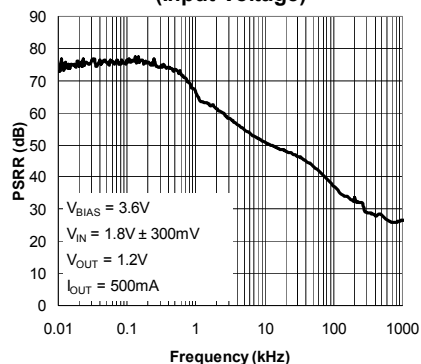
Power Supply Ripple Rejection (Input Voltage)
