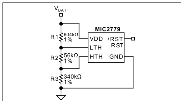
FIGURE 4-1: Example Circuit.
