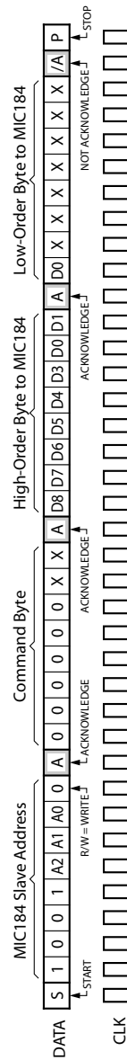
Figure 3. WRITE_WORD Protocol
