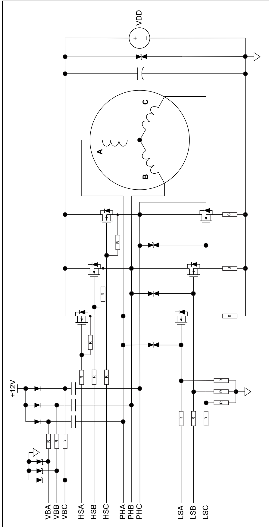
Figure 5-3 shows the location of the overvoltage TVS devices, bootstrap resistors and gate-to-source resistors.
