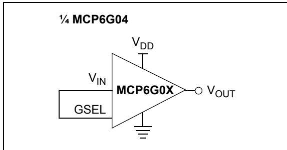
FIGURE 4-8: Unused Amplifiers.
