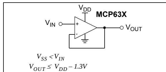
FIGURE 4-3: Unity-Gain Voltage Limitations for Linear Operation.
