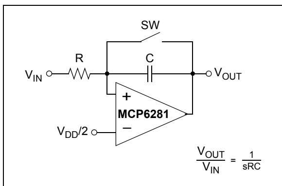
FIGURE 4-9: Miller Integrator.
