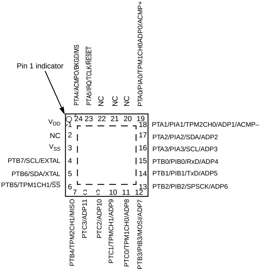
Figure 2-1. 24-Pin QFN
