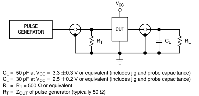
Figure 4. Test Circuit
