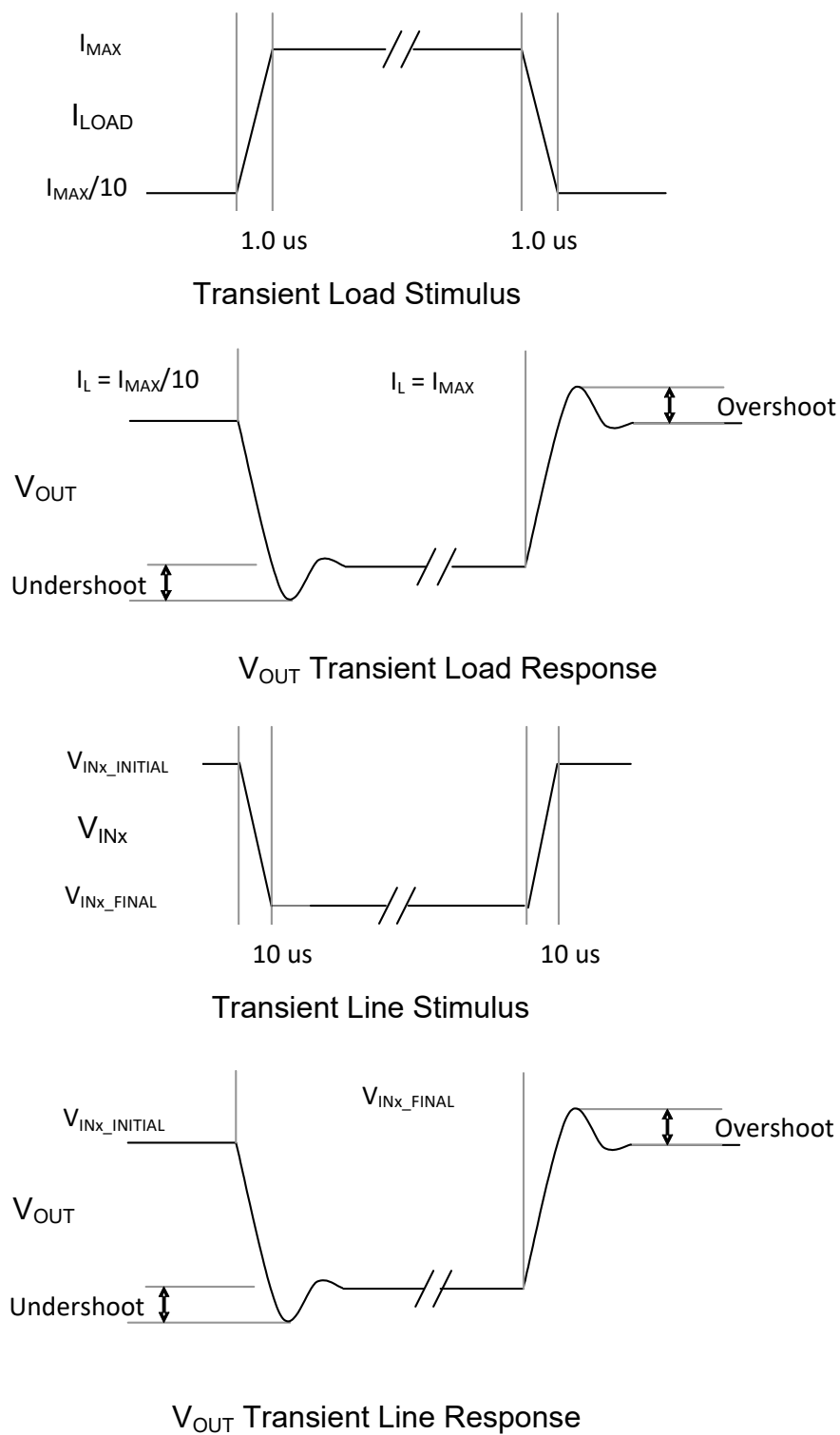
Figure 25. Transient waveforms
