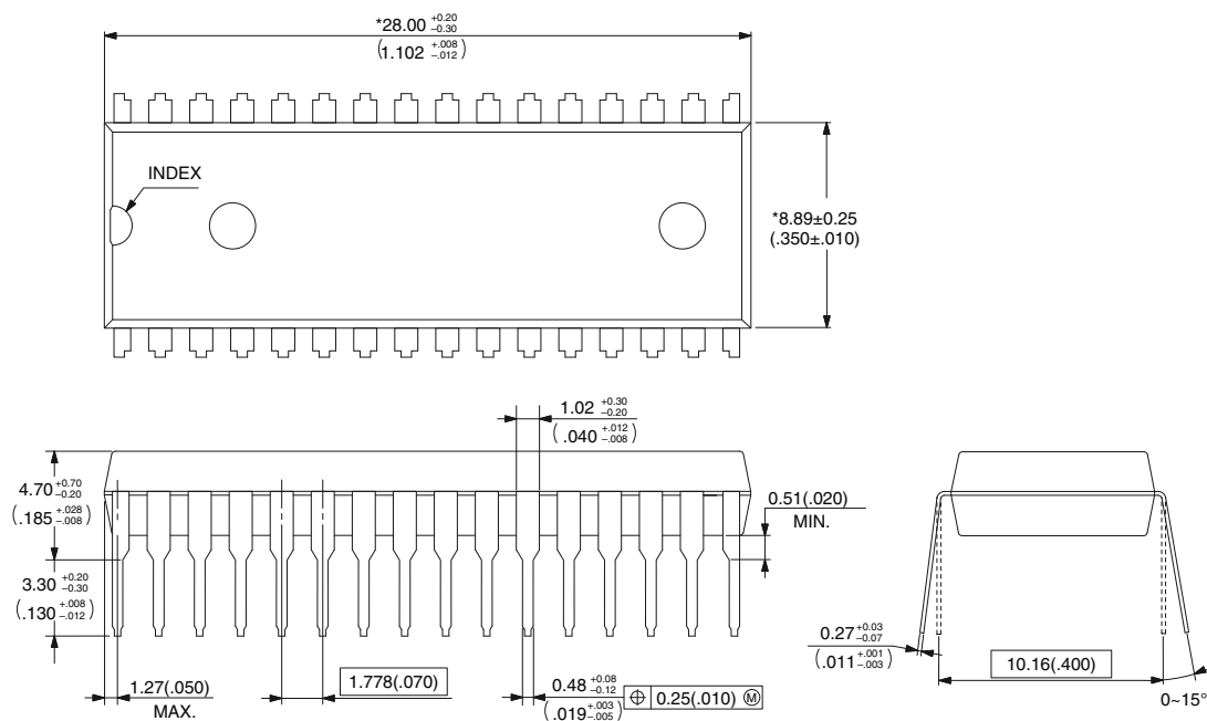
Note 1) * : These dimensions do not include resin protrusion. Note 2) Pins width and pins thickness include plating thickness.
