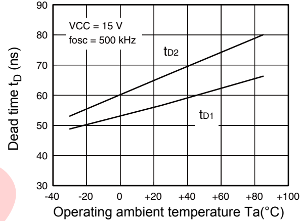
Dead time vs. Operating ambient temperature
