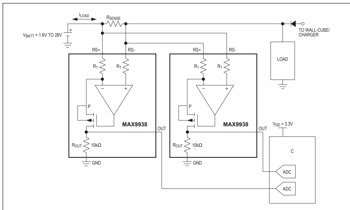
Figure 3. Bidirectional Application
