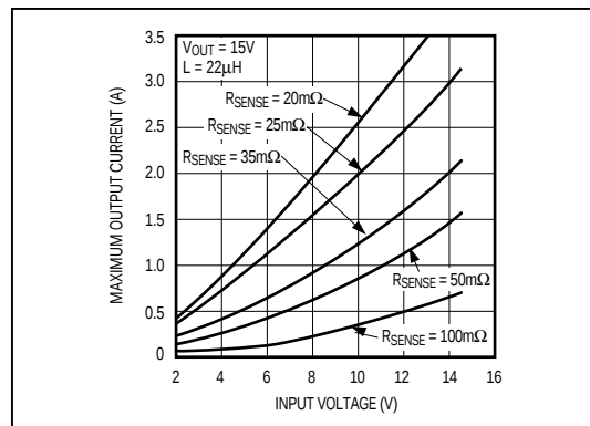
Figure 4d. Maximum Output Current vs. Input Voltage ( V_{OUT} = 15V )
