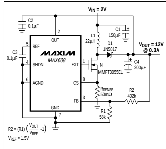
Figure 2b. 12V Output
