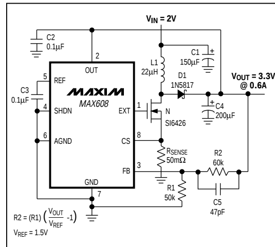
Figure 2c. 3.3V Output
