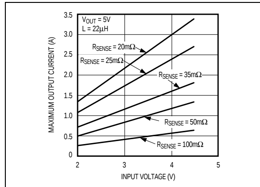
Figure 4b. Maximum Output Current vs. Input Voltage ( V_{OUT} = 5V )
