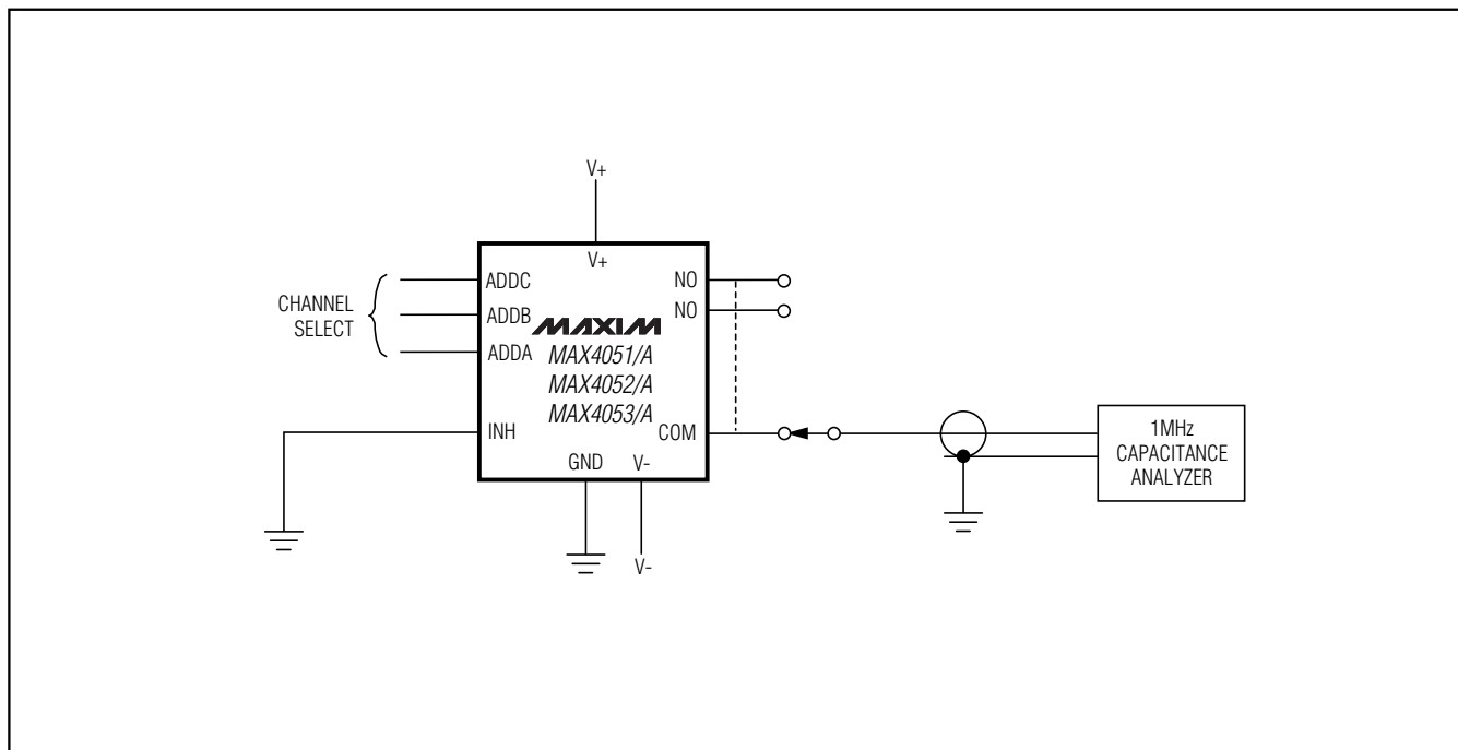
Figure 7. NO/COM Capacitance
