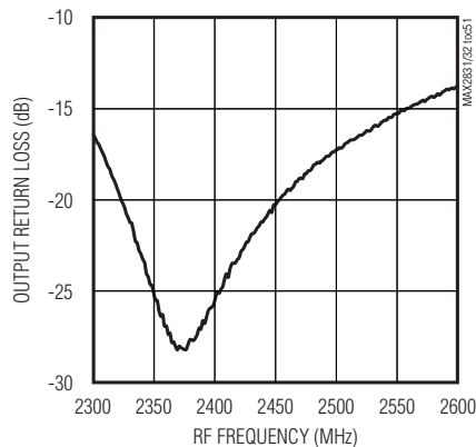
PA OUTPUT RETURN LOSS vs. RF FREQUENCY
