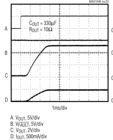
STARTUP WAVEFORMS C_{OUT} = 330\mu F
