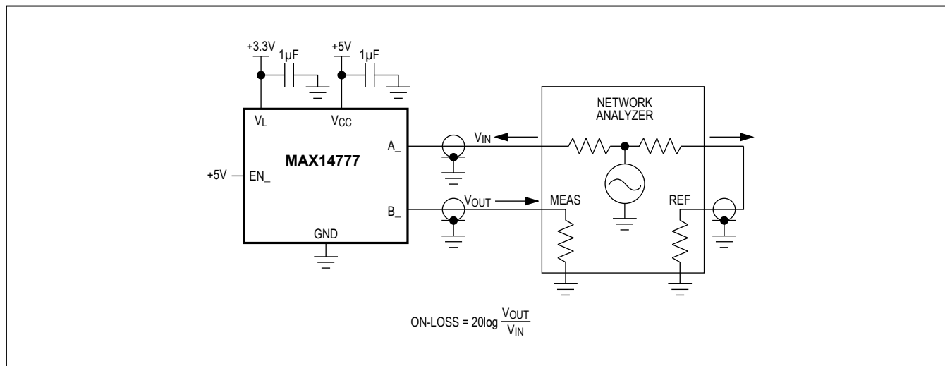
Figure 6. Frequency Response
