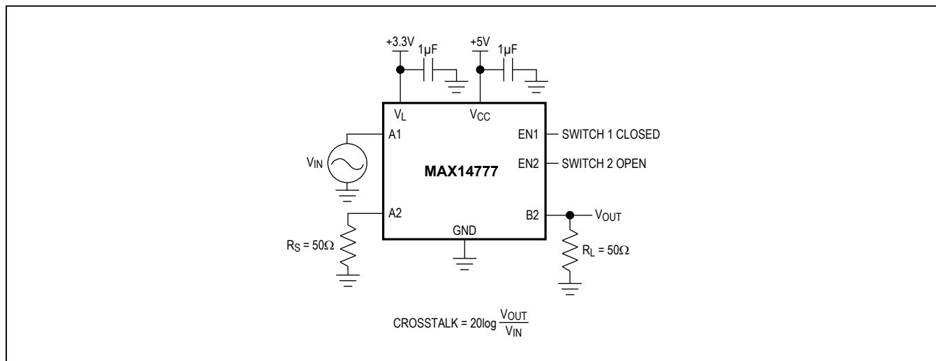
Figure 5. Crosstalk
