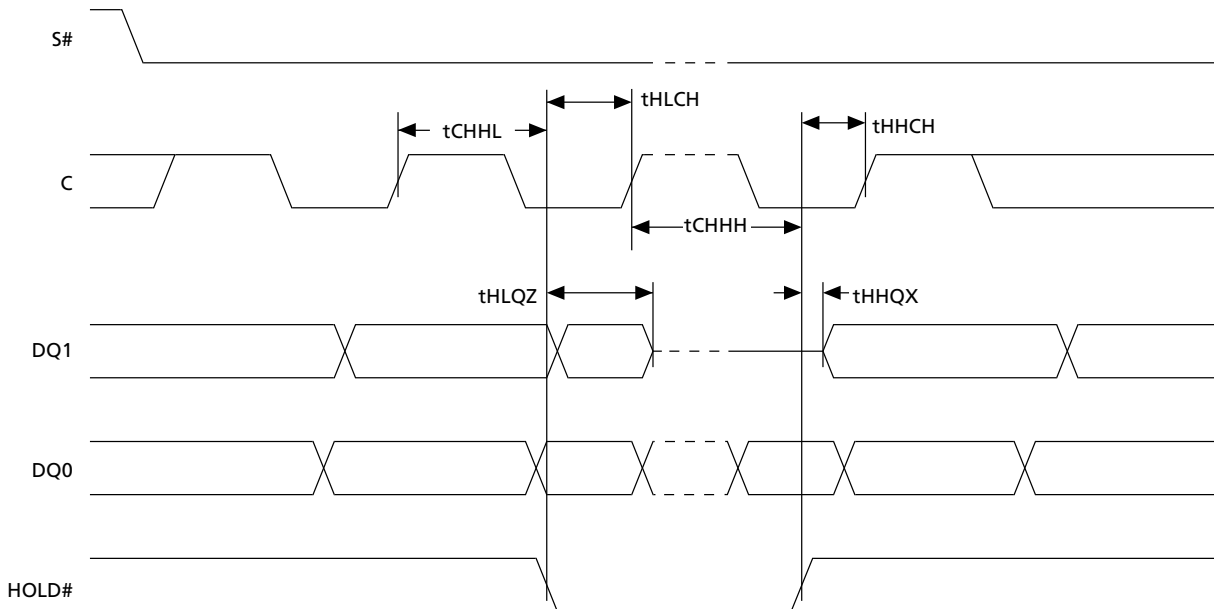
Figure 27: Hold Timing
