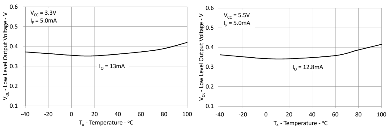
Figure 5: Typical Low Level Output Voltage vs. Ambient Temperature
