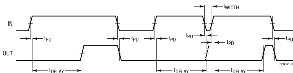
Figure 3. Rising-Edge Delayed Timing Diagram (LTC6994-1, \text{POL} = 0 )
