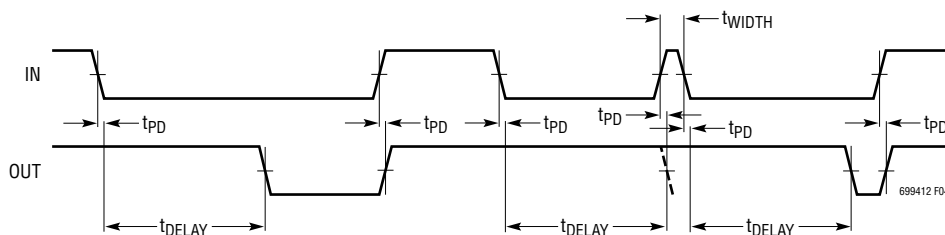
Figure 4. Falling-Edge Delayed Timing Diagram (LTC6994-1, \text{POL} = 1 )
