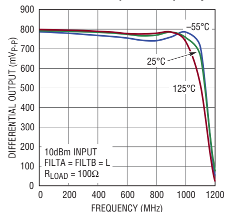
Differential Output vs Frequency
