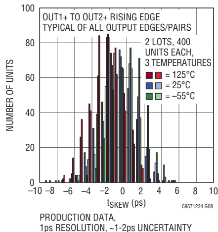
Typical Distribution of Skew
