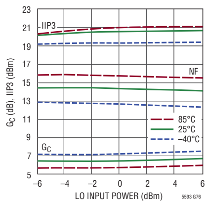
3200MHz Conversion Gain, IIP3 and NF vs LO Power
