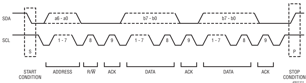
Figure 11. Data Transfer over I 2 C or SMBus
