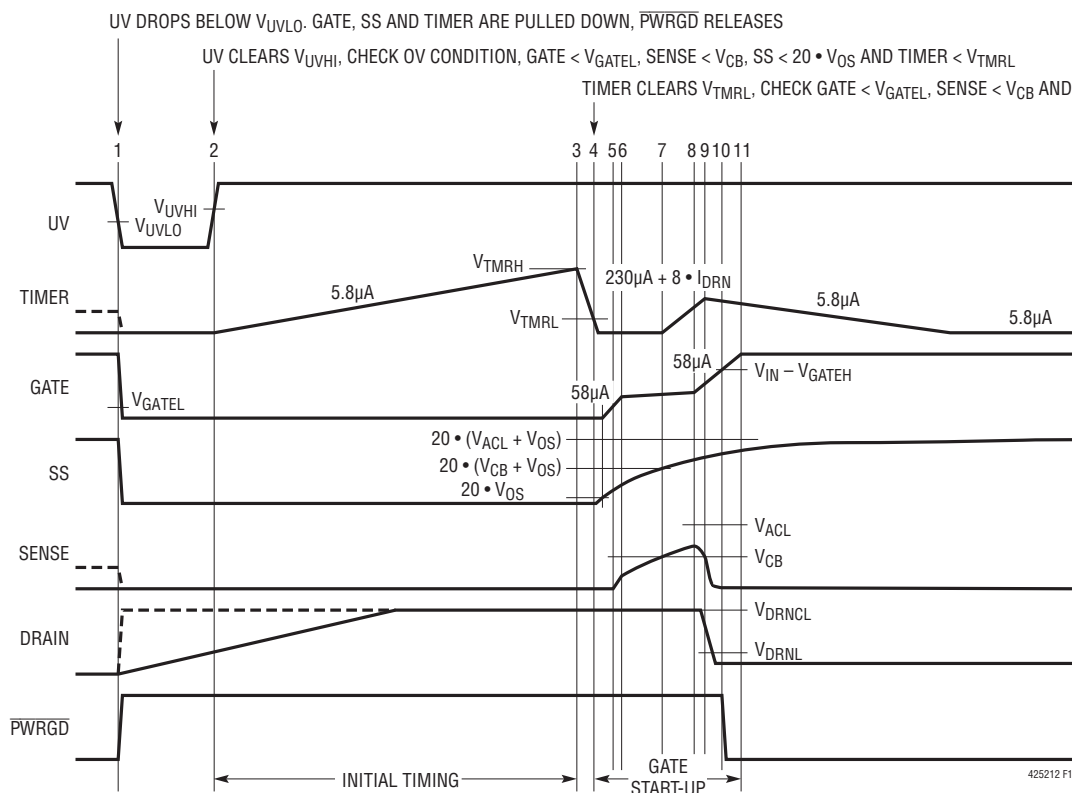
Figure 11. Undervoltage Timing (All Waveforms Are Referenced to V_{EE} )
