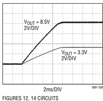
Soft Start-Up
