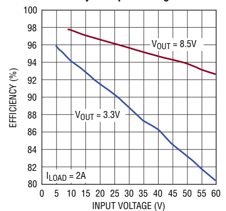
FIGURES 12, 14 CIRCUITS
