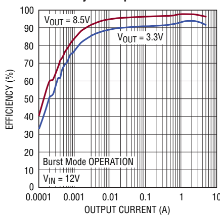
FIGURES 12, 14 CIRCUITS
