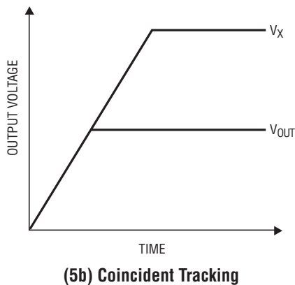
Figure 5b and 5c. Two Different Modes of Output Voltage Tracking
