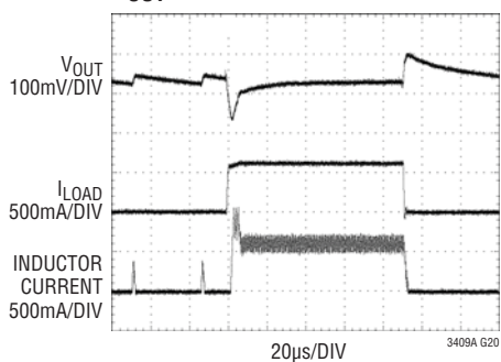
Load Step 10mA to 600mA, Burst Mode Operation, V_{IN} = 3.6\text{V} , V_{OUT} = 1.8\text{V}
