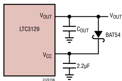
Figure 6. Example of V_{CC} Bootstrap
