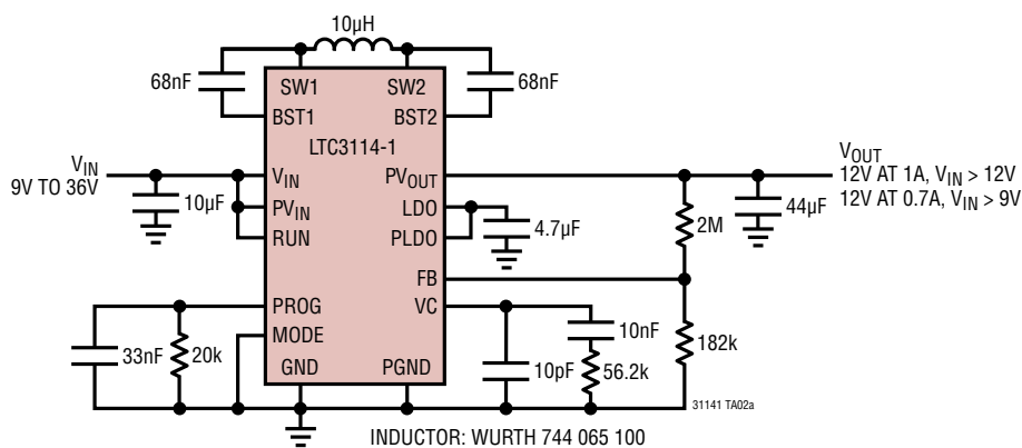
9V to 36V V_{IN} to 12V V_{OUT} Regulator
