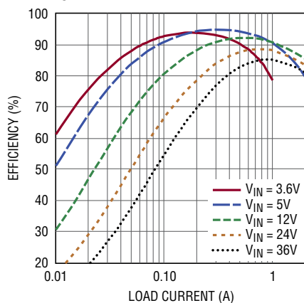
PWM Mode Efficiency, V_{OUT} = 5\text{V} , f_{SW} = 500\text{kHz} , Non-Bootstrapped
