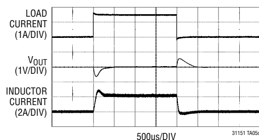
0A to 1.5A Load Step, V_{IN} = 20V
