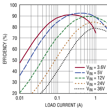
PWM Mode Efficiency, V_{OUT} = 5\text{V} , f_{SW} = 1\text{MHz} , Non-Bootstrapped
