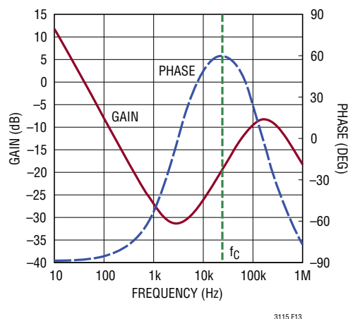
Figure 13. Compensated Error Amplifier Bode Plot
