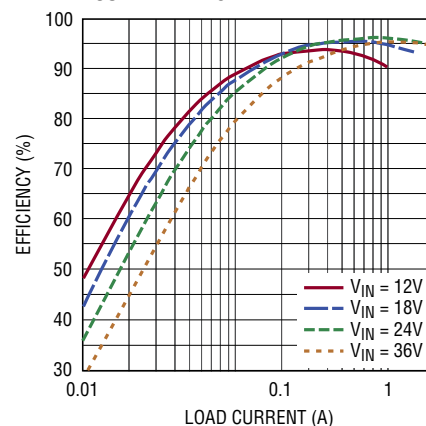
PWM Mode Efficiency, V_{OUT} = 24\text{V} , f_{SW} = 500\text{kHz}
