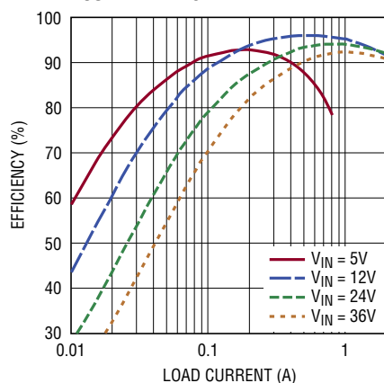
PWM Mode Efficiency, V_{OUT} = 12\text{V} , f_{SW} = 500\text{kHz}
