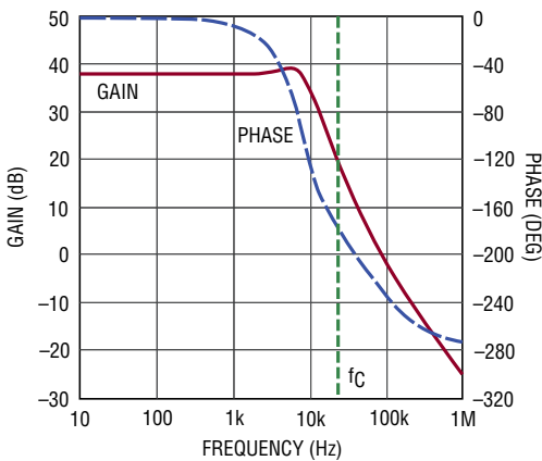
Figure 12. Converter Bode Plot, V_{IN} = 3.5V , I_{LOAD} = 500mA
