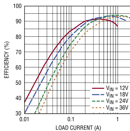
PWM Mode Efficiency, V_{OUT} = 24\text{V} , f_{SW} = 1\text{MHz}
