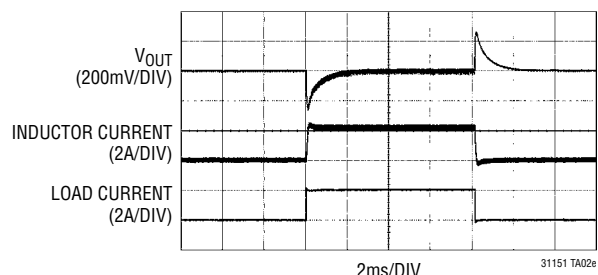
V OUT Transient for a 0A to 2A Load Step, V IN = 24V
