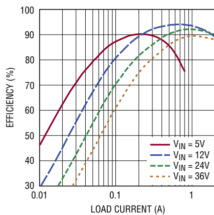
PWM Mode Efficiency, V_{OUT} = 12\text{V} , f_{SW} = 1\text{MHz}
