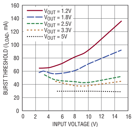
Automatic Burst Mode Threshold vs Supply Voltage
