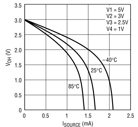
\overline{\text{RST}} High Level Output Voltage vs Output Source Current (LTC2902-2)
