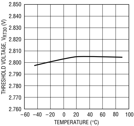
3V Threshold Voltage vs Temperature
