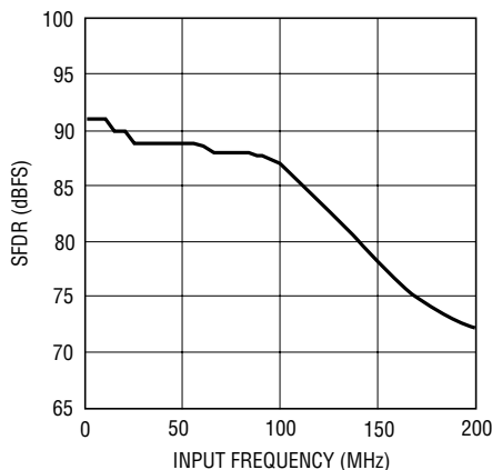
LTC2286: SFDR vs Input Frequency, -1\text{dB} , 2V Range, 25Msps
