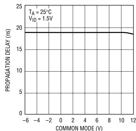
Propagation Delay vs Common Mode
