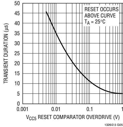
V_{CC5} Transient Immunity (LTC1326)
