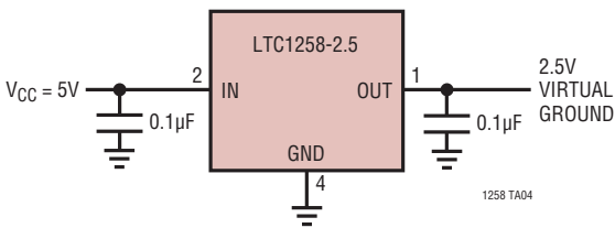
Supply Splitter
