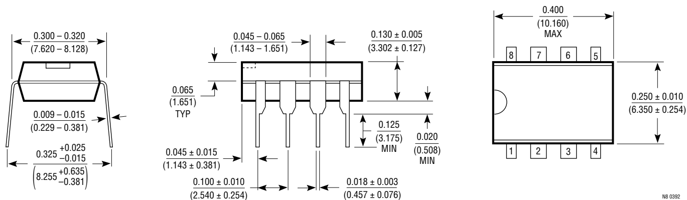
N8 Package 8-Lead Plastic Lead
