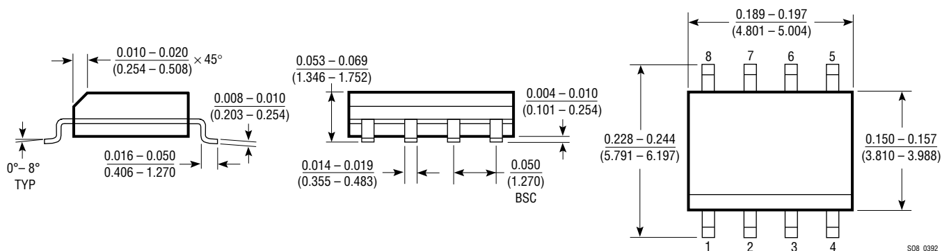
S8 Package 8-Lead Plastic SOIC
