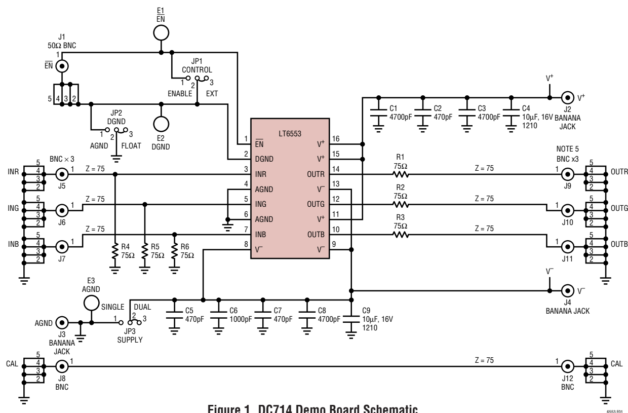
Figure 1. DC714 Demo Board Schematic
