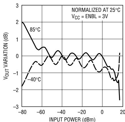
V_{OUT} Variation vs Input Power at 200MHz
