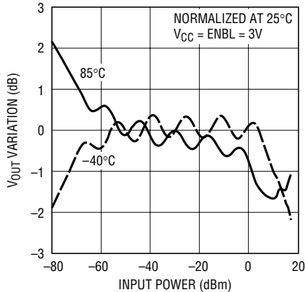
V_{OUT} Variation vs Input Power at 50MHz
