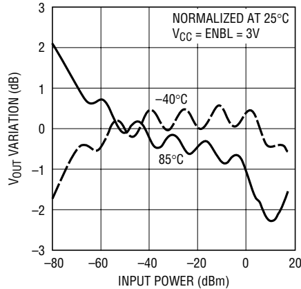
V_{OUT} Variation vs Input Power at 10MHz
