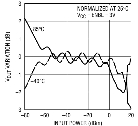
V_{OUT} Variation vs Input Power at 100MHz
