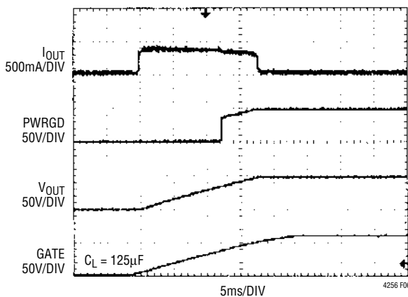
Figure 6. Start-Up Waveforms
