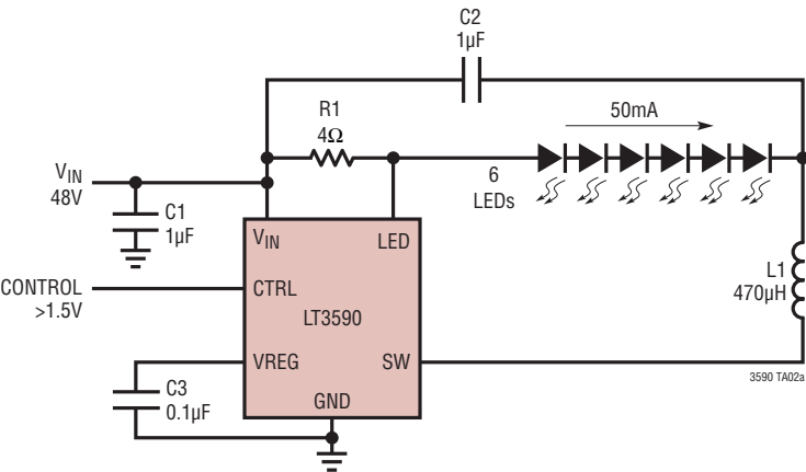
48V Supply for 6 LED String, 50mA Current
