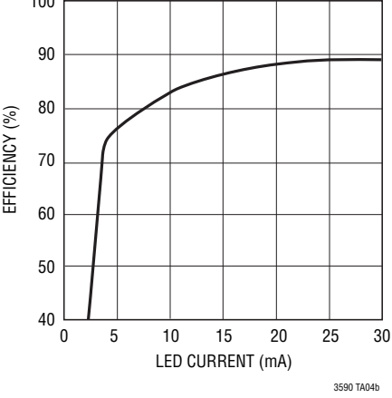
Conversion Efficiency
