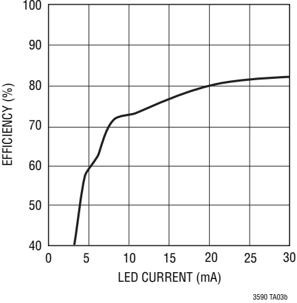
Conversion Efficiency
