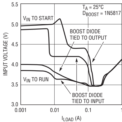
Minimum Input Voltage, V_{OUT} = 3.3V (LT3506A)
