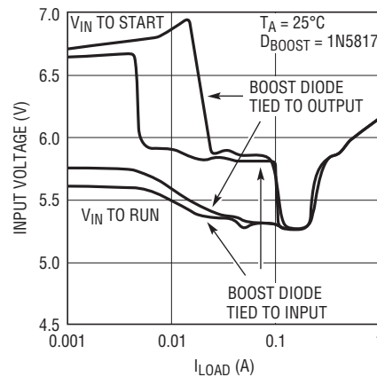
Minimum Input Voltage, V_{OUT} = 5V (LT3506A)
