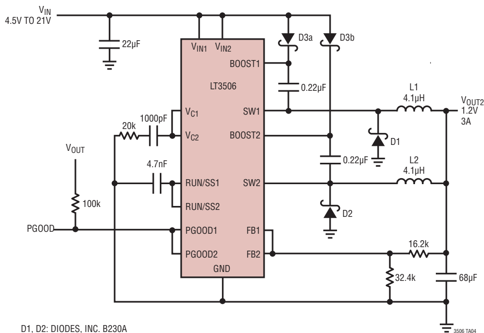
Low Ripple, Low Profile 1.2V, 3A Converter, Maximum Height = 2mm
