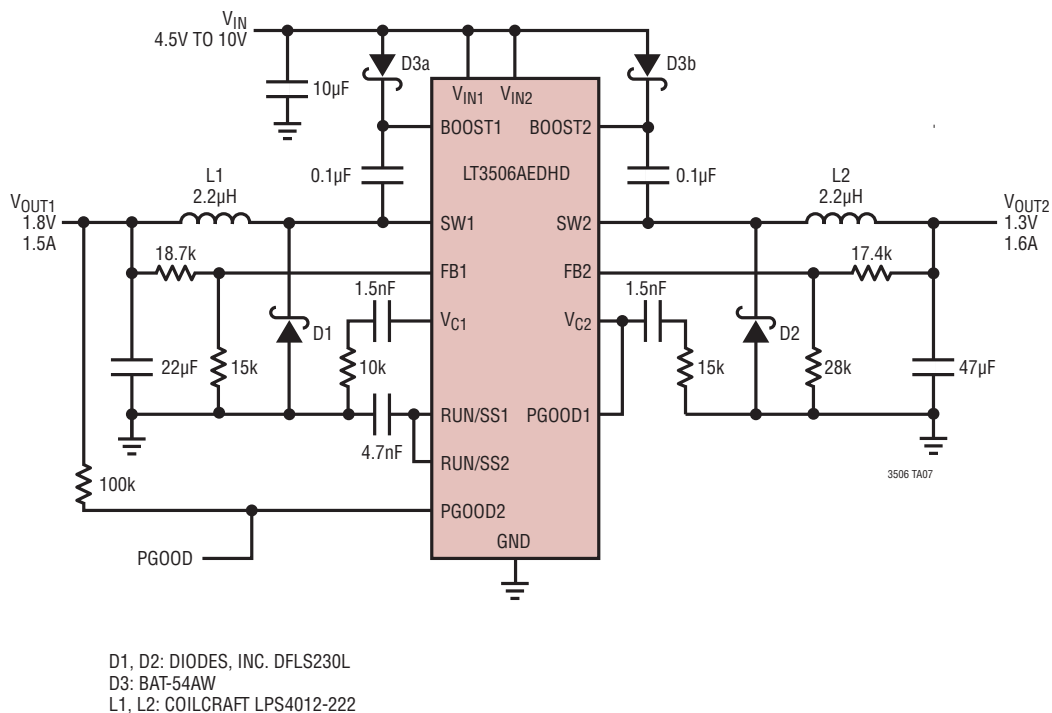
Low Profile 1.8V and 1.3V Outputs with Sequencing, Maximum Height = 1.2mm
