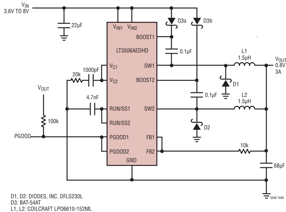
Low Ripple, Low Profile 0.8V, 3A Converter, Maximum Height = 1mm
