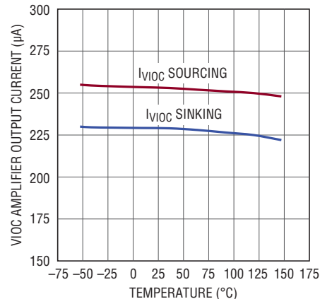
VIOC Amplifier Output Current vs Temperature
