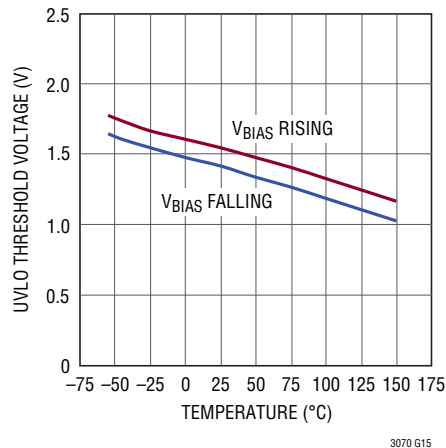
BIAS Pin Undervoltage Lockout Threshold
