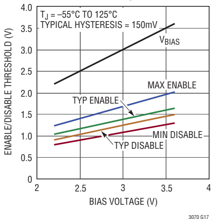
Enable Pin Threshold and Hysteresis vs V_{BIAS}
