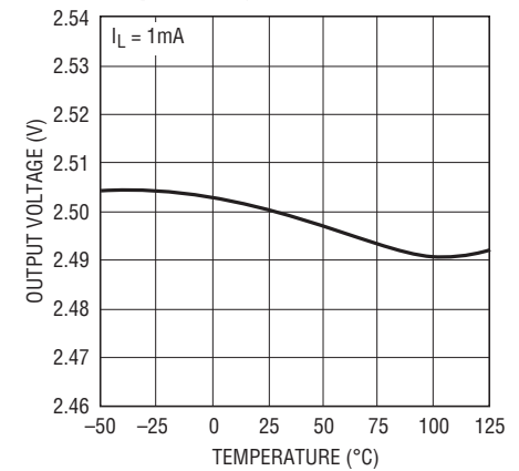
LT1761-2.5 Output Voltage
