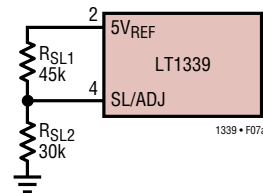
Figure 7a. External Slope Compensation Resistors
